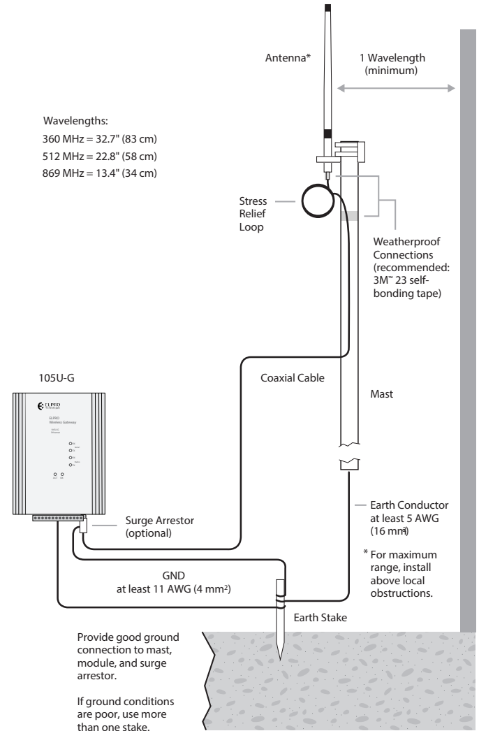
Figure 1. Antenna Installation
