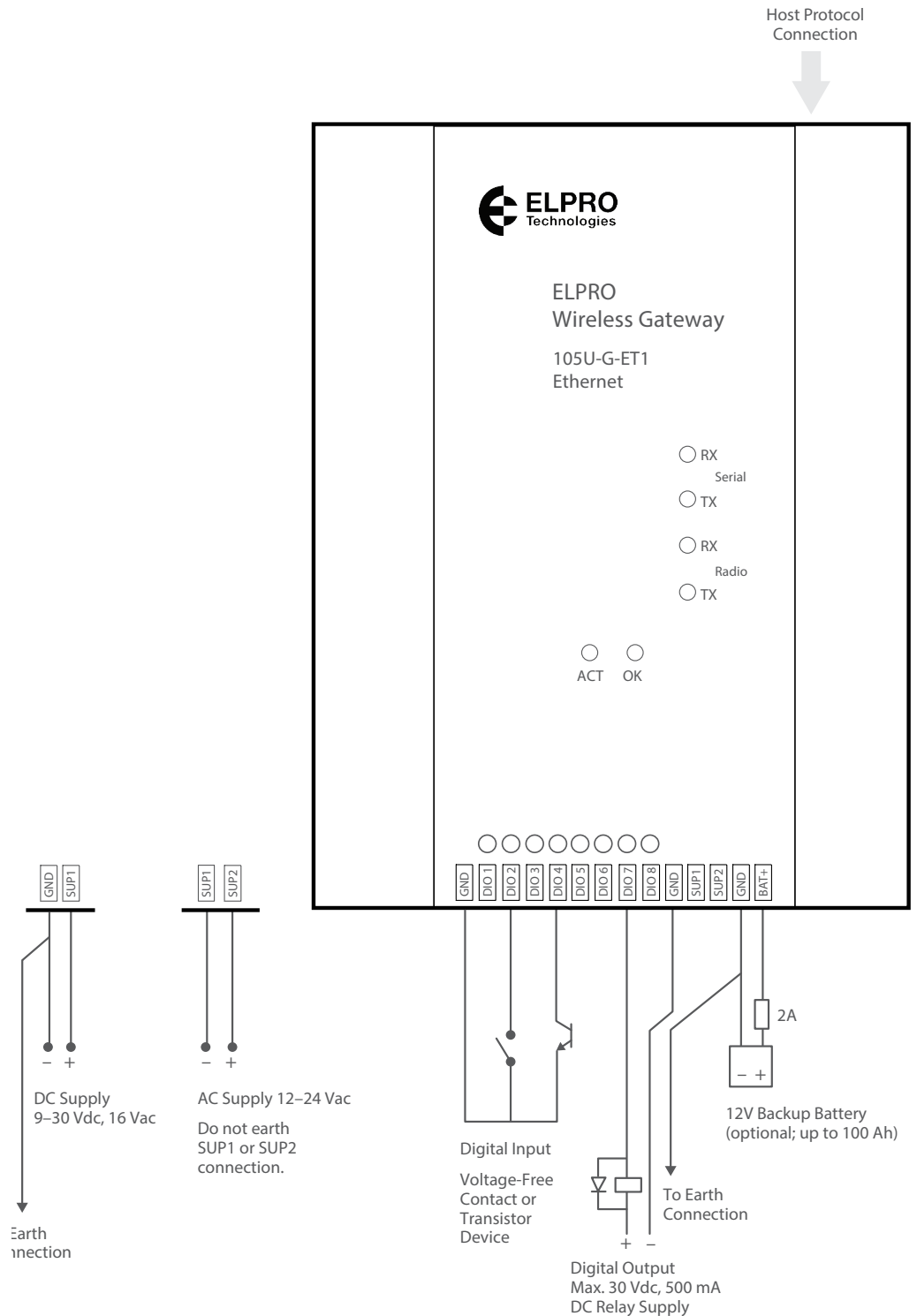
Figure 2. Wiring Diagram
