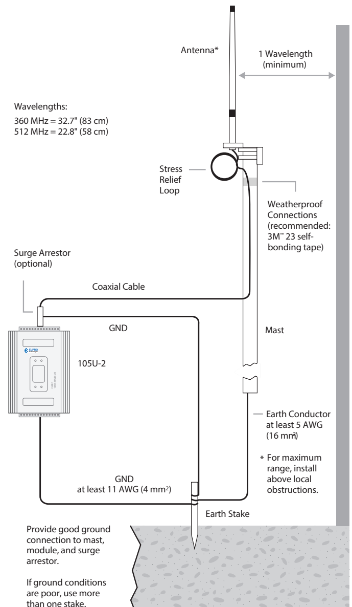
Figure 1. Antenna Installation
