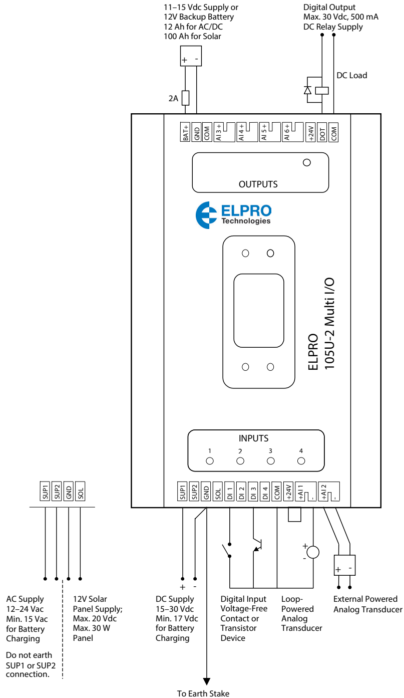
Figure 2. Wiring Diagram
